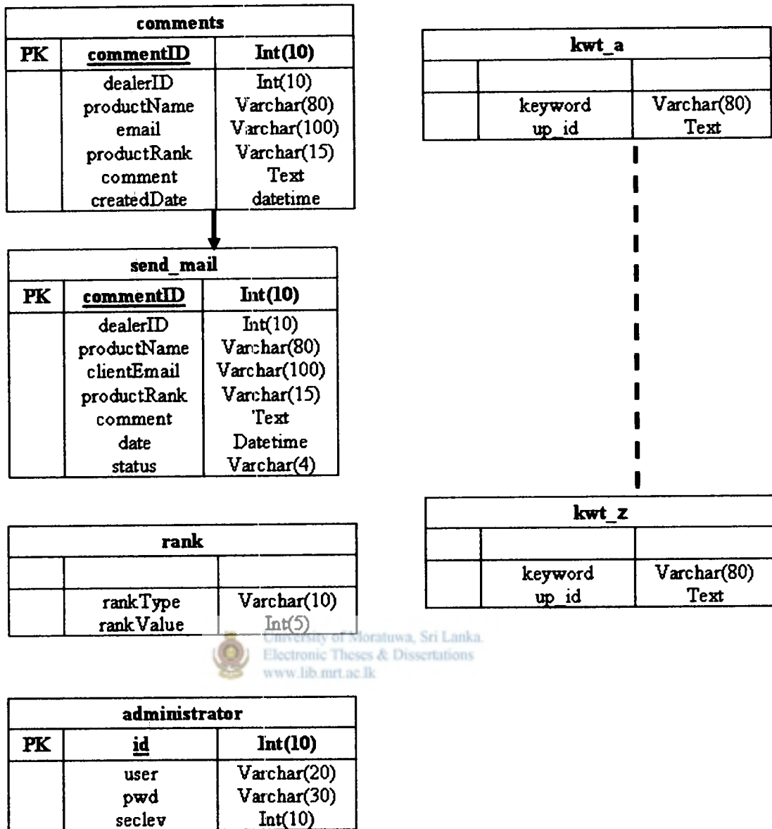
Figure 1: Entity Integrity Diagram A
