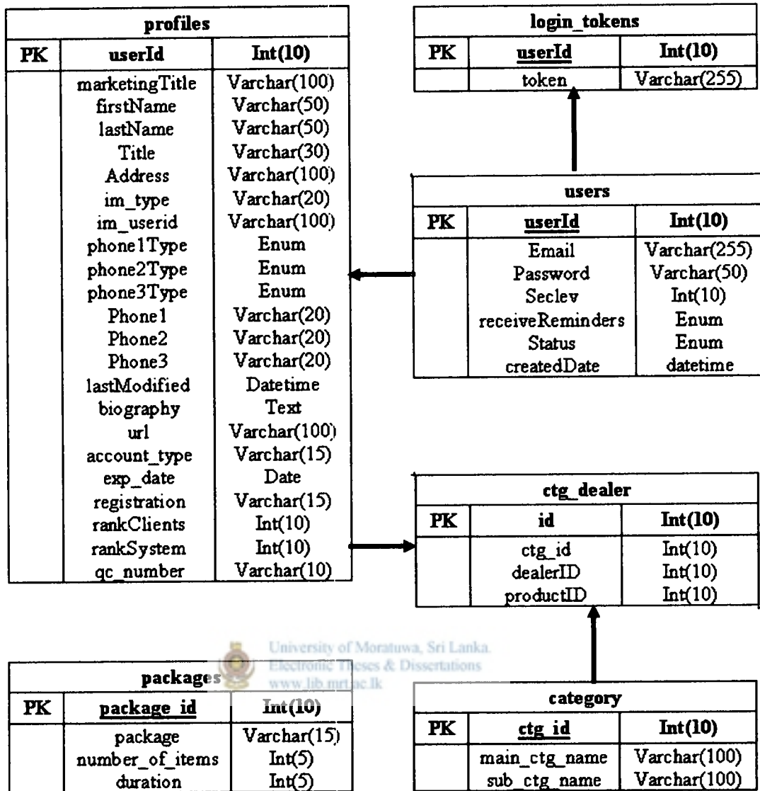
Figure 2: Table Relationship Diagram B
