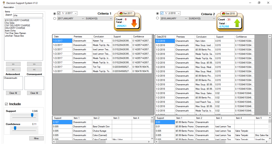
Figure 7.5 – System User interface
