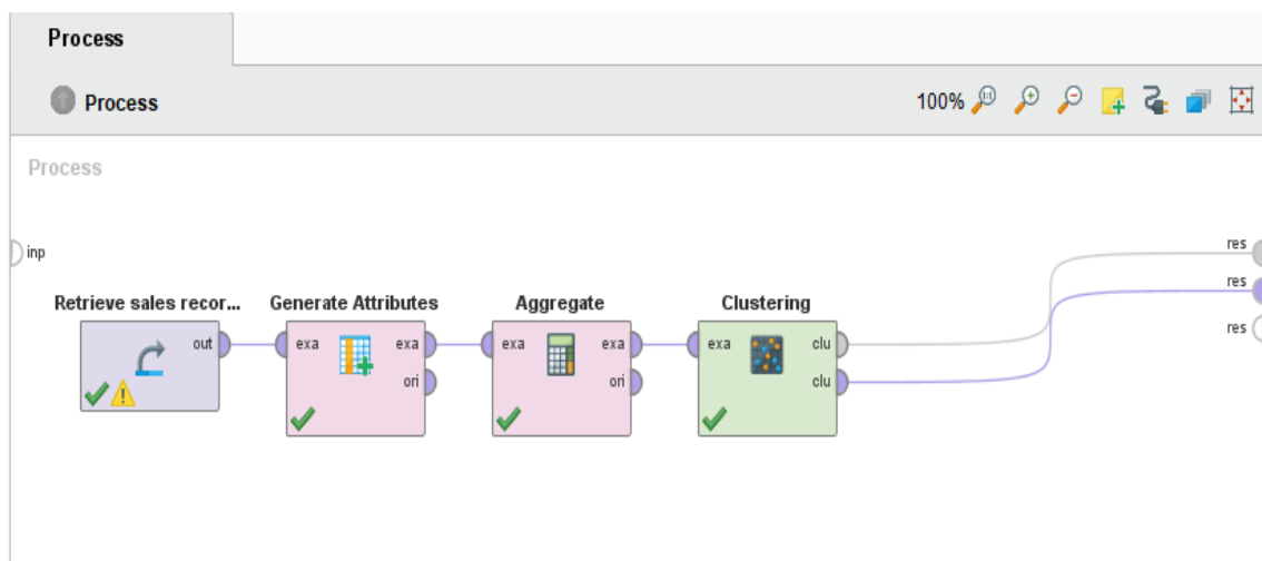
Figure 6.06 Clustering diagram
