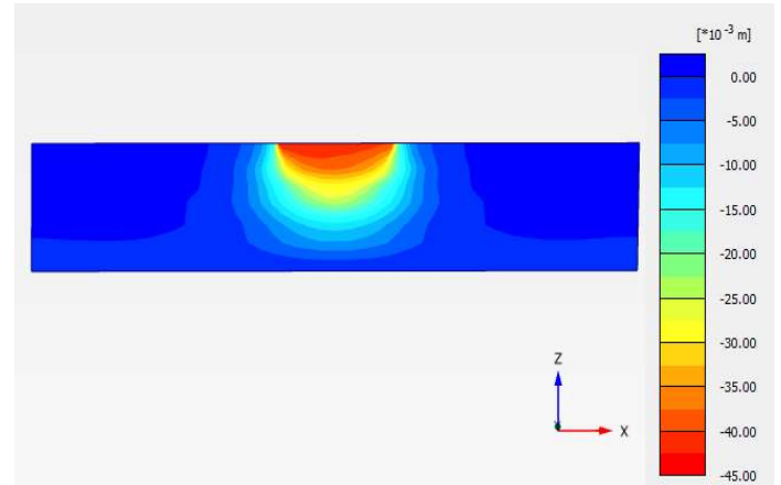
Settlement of oil storage tank foundation for D'=14.0\text{m} , q=149.46\text{kN/m}^2
