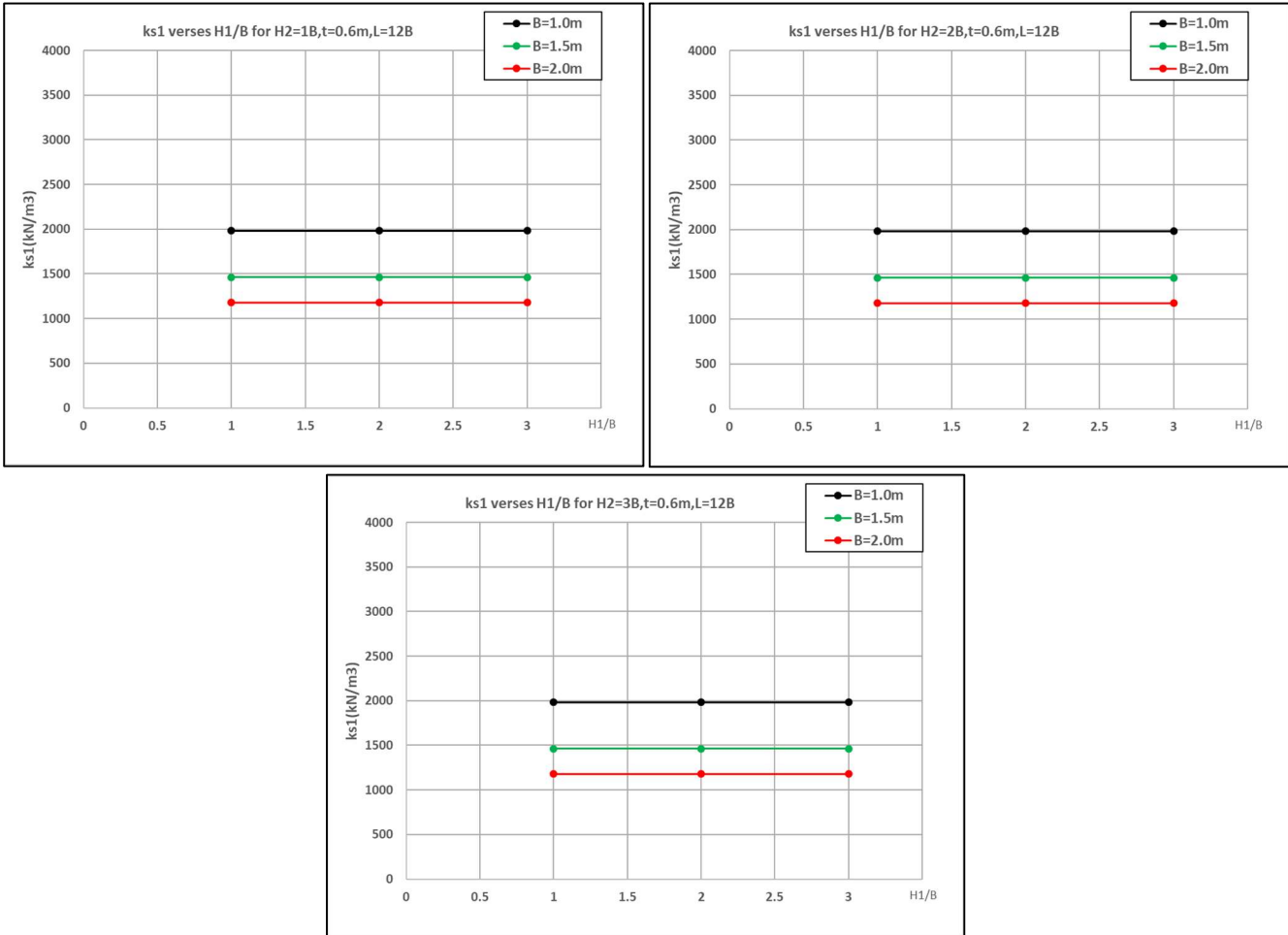
Figure 4. 2: Equivalent spring theory equivalent subgrade modulus k_{s1} versus H_1/B for t=0.6m
