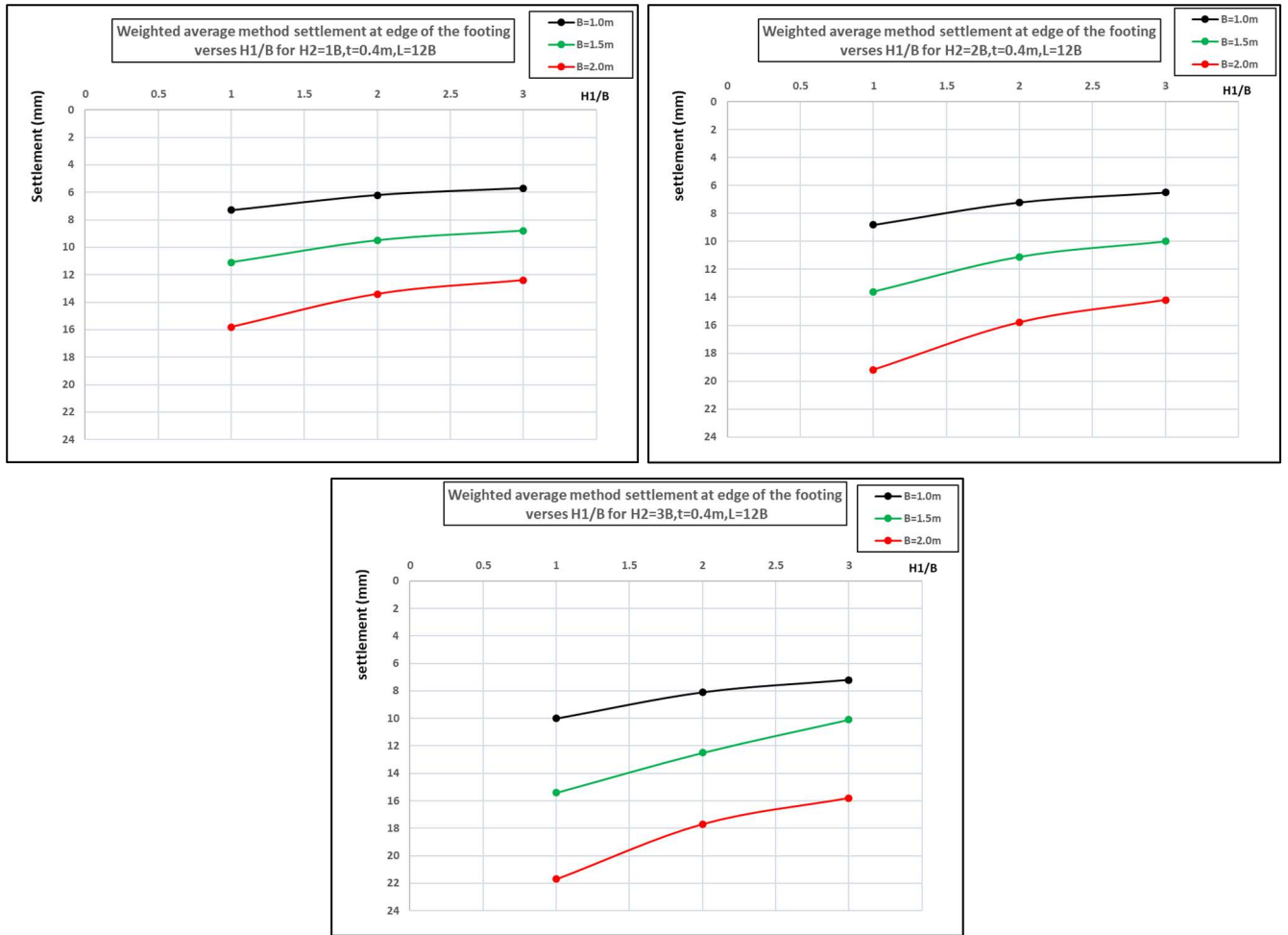
Figure 4. 10: Weighted average method settlement at edge of the footing versus H_1/B for t=0.4m
