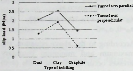
Figure 3 - Variation of the slip load with infillings.
