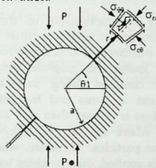
Figure 4 - An inclined, radially oriented pale of weakness intersecting a circular excavation
