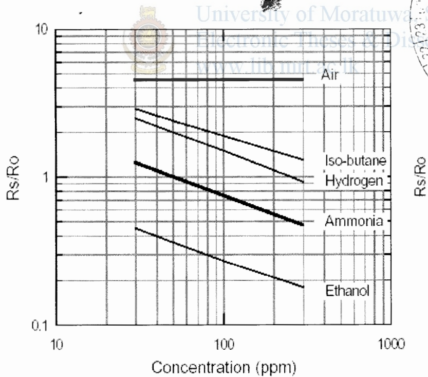
Appendix 2: Sensitivity characteristics of the ammonia sensor.
