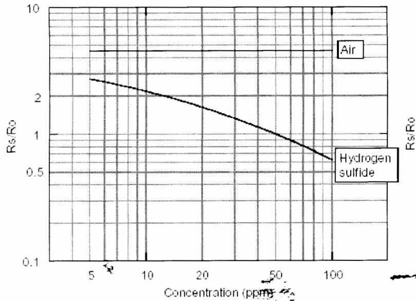
Appendix 1: Sensitivity characteristics of the hydrogen sulfide sensor
