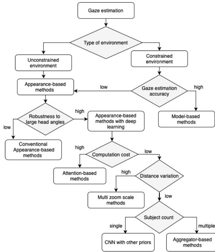
Figure 15: Guide to select a deep learning-based gaze estimation approach.
