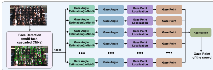
Figure 13: Representation of the model architecture by Kodama et al. (2018).
