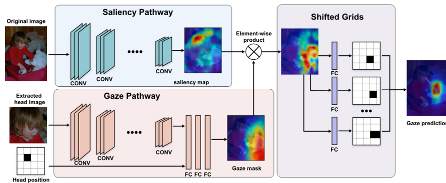
Figure 10: Representation of the GazeFollow network architecture presented by Recasens (2016).
