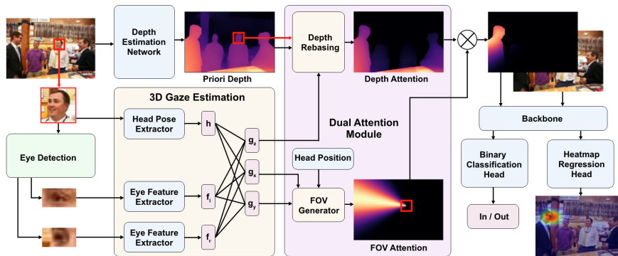
Figure 9: Representation of the model architecture presented by Fang et al. (2021).
