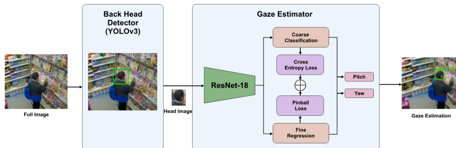
Figure 14: Representation of the EyeShopper system architecture by Bermejo et al. (2020) .
