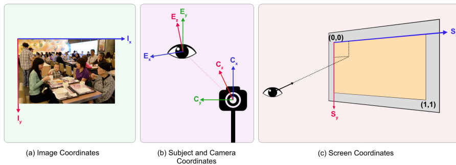
Figure 7: Coordinate systems used for 2D and 3D gaze estimation; (a) Image coordinates, (b) Subject and camera coordinates, (c) Screen coordinates.
