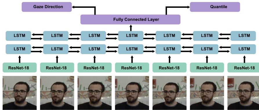
Figure 12: Representation of the Gaze360 model architecture by Kellnhofer et al. (2019).
