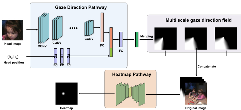
Figure 11: Representation of the model architecture presented by Lian et al. (2018).
