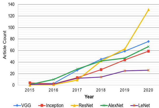
Figure 2: Evolution of deep Learning-based gaze estimation techniques.
