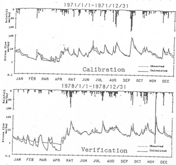
Fig 2 Observed and Calculated Hydrographs
