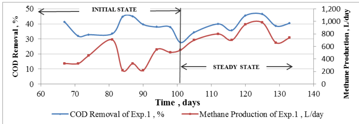
Figure 3: COD Removal Efficiency and Methane Production of Exp1
