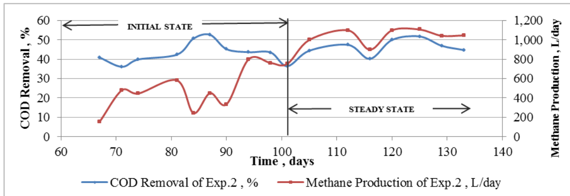
Figure 4: COD Removal Efficiency and Methane Production of Exp
