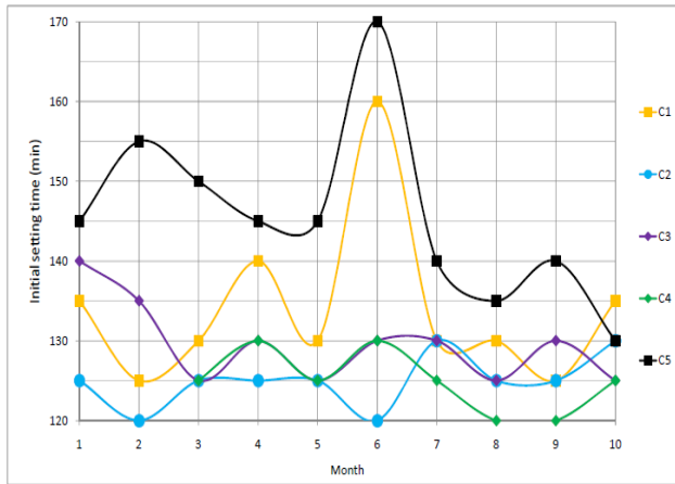
Fig. 6 Initial Setting time
