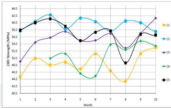
Fig. 4 28day (28D) strength of Mortar samples
