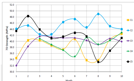
Fig. 3 7day (7D) strength of Mortar samples
