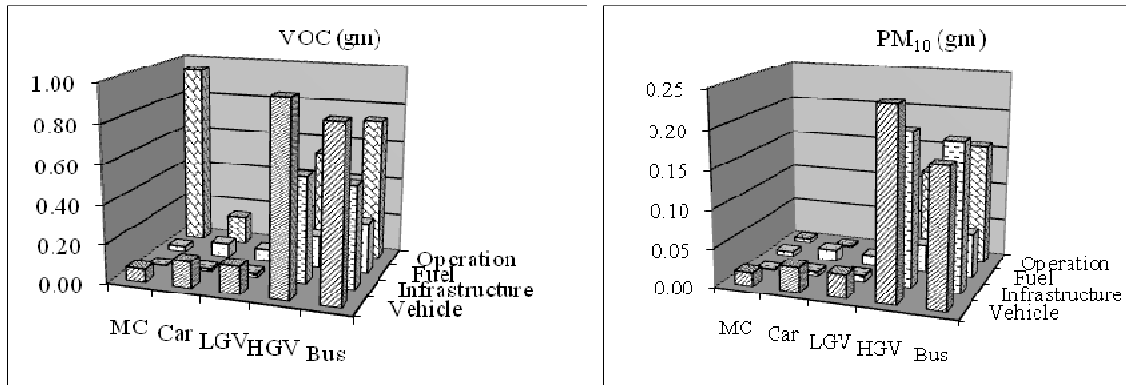
Figure 3 Pollutant emissions (by mode and LCA phase of road transport) per VKT
