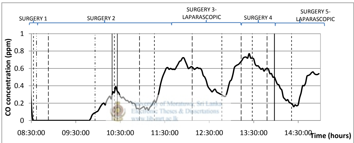
Figure 10: CO Concentration inside the Theatre
