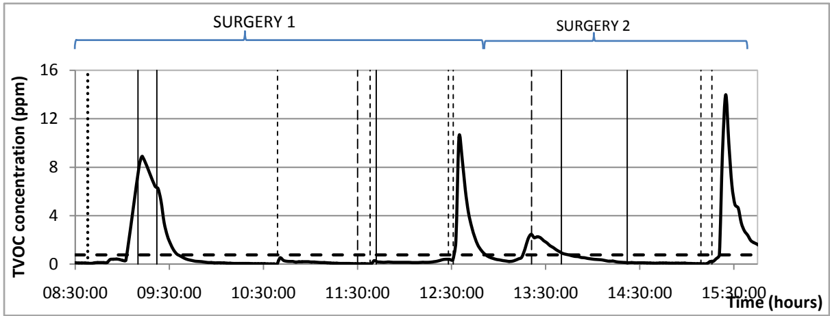
Figure 9: TVOC Concentration inside the Theatre
