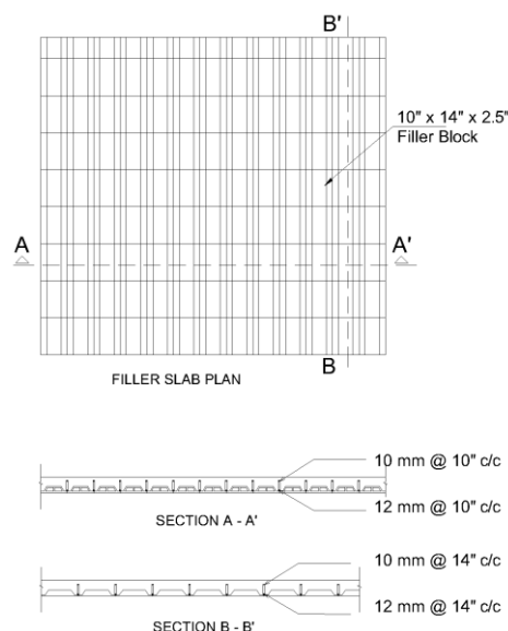
Figure 2: Typical plan and section of a filler slab with hollow filler clay block
