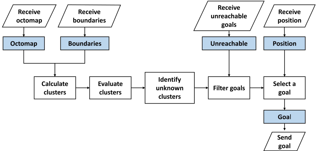
Figure 4.7: Exploration module during multi-robot operation
