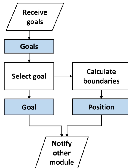
Figure 4.15: Data received by the client module is used to update other modules
