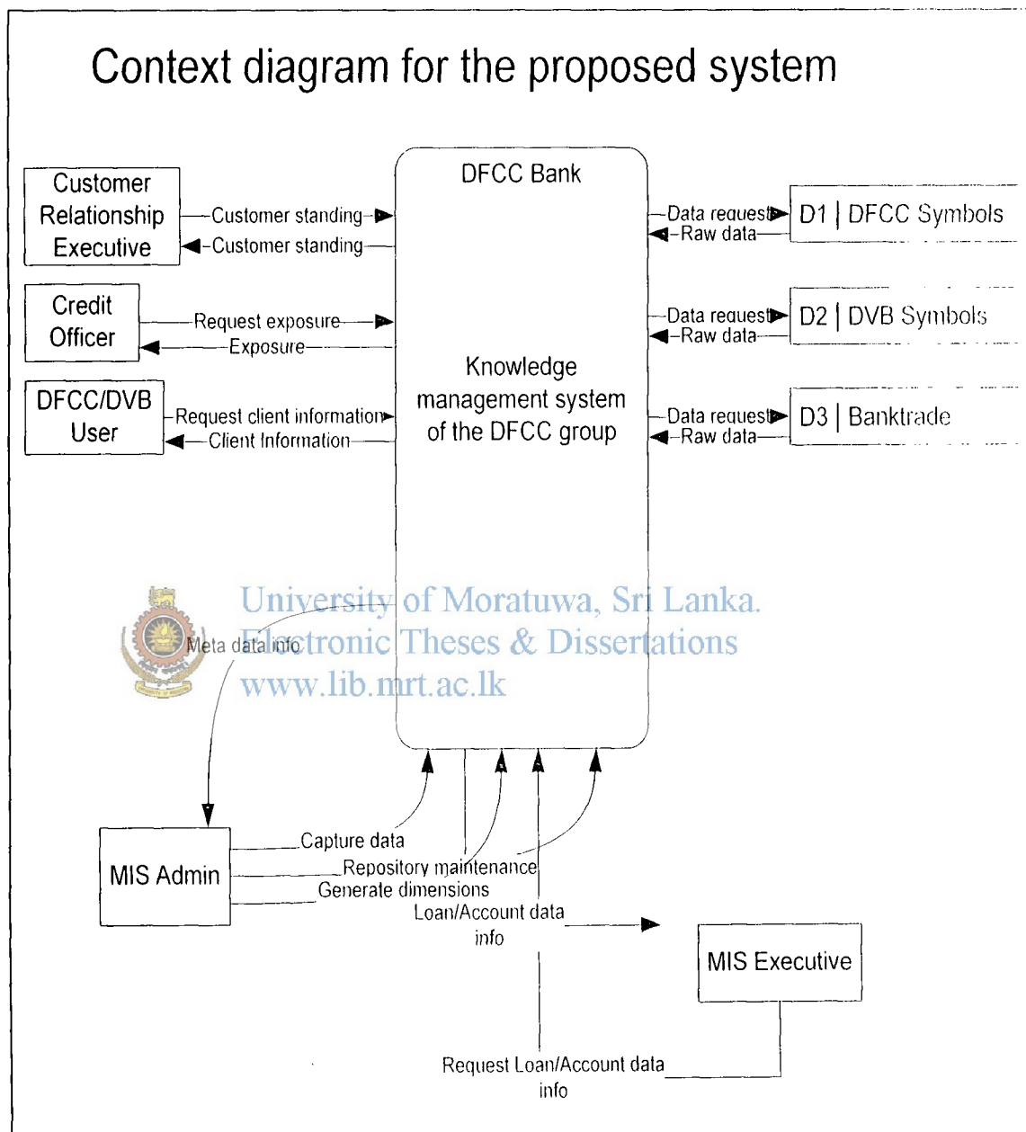
Context diagram for the proposed system
