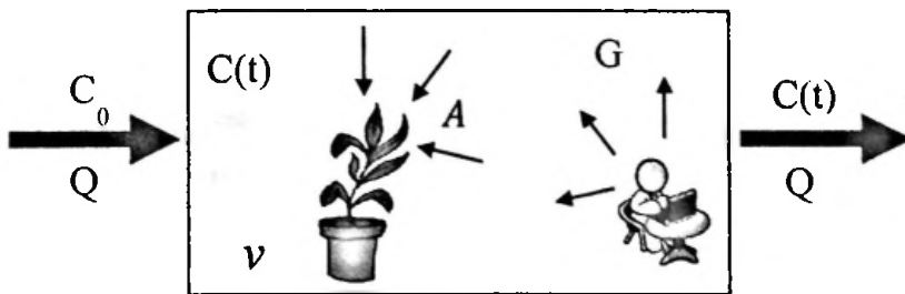
Figure 3.3: Mass balance of CO 2 inside a mechanically ventilated room with indoor plants
