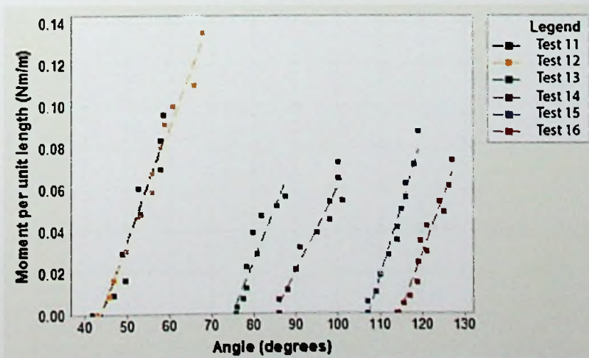
Figure 3.9: Moment - angle relationship for Kapton 300HN (75 \mu\text{m} )
