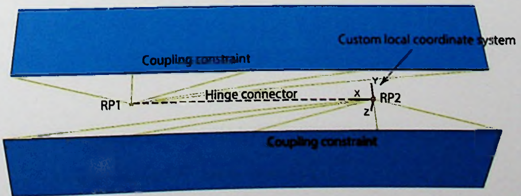
Figure 4.4: Coupling constraint with hinge connector
