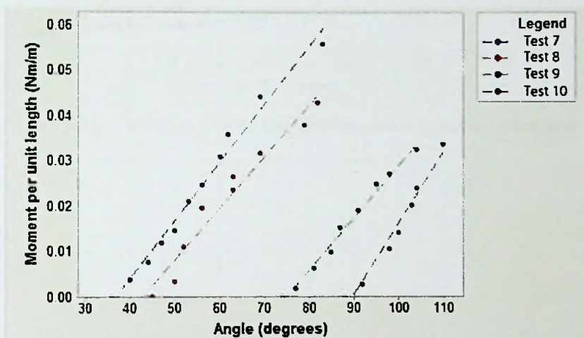
Figure 3.8: Moment - angle relationship for Kapton 200HN (50 \mu\text{m} )
