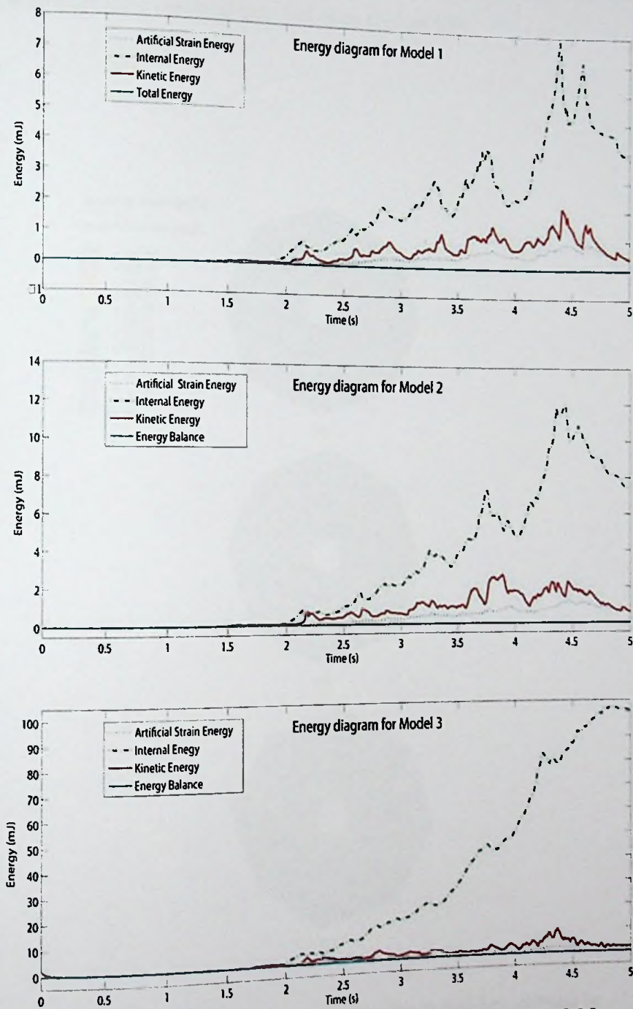
Figure 5.6: Energy plots recorded for model 1, model 2 and model 3
