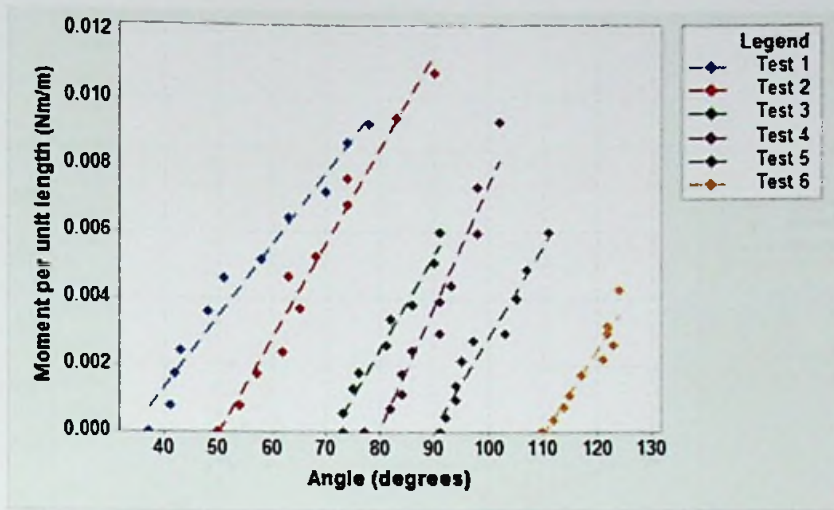
Figure 3.7: Moment - angle relationship for Kapton 100HN (25 \mu\text{m} )
