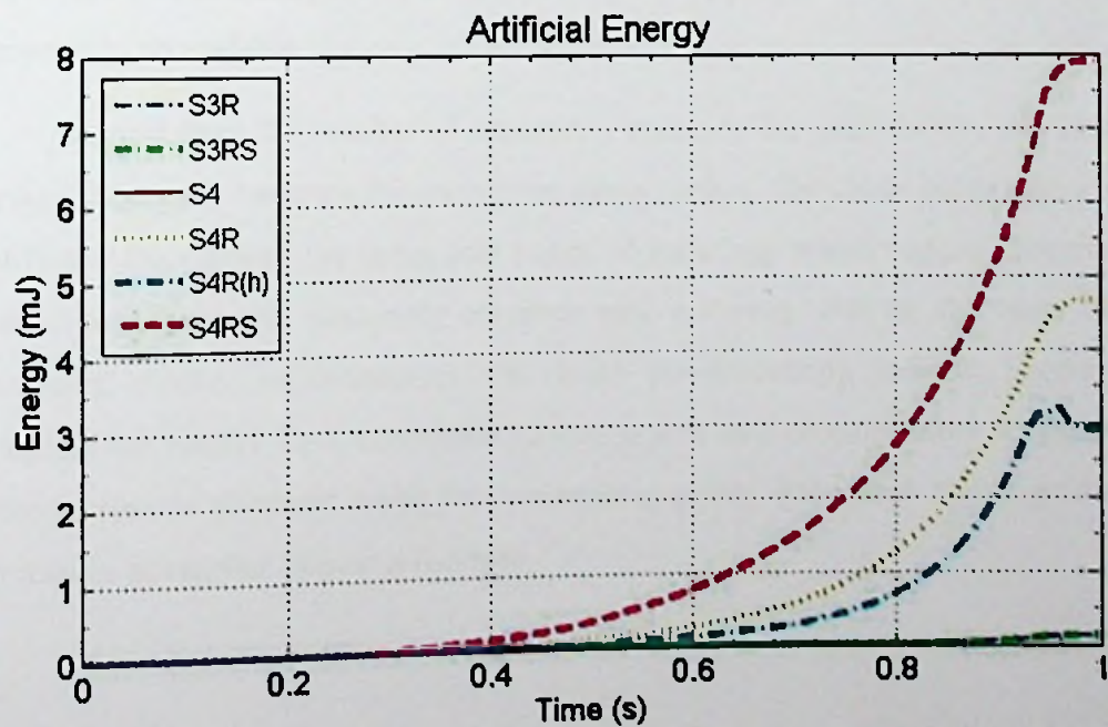
Figure 4.5: Artificial energy diagram for conventional shell elements
